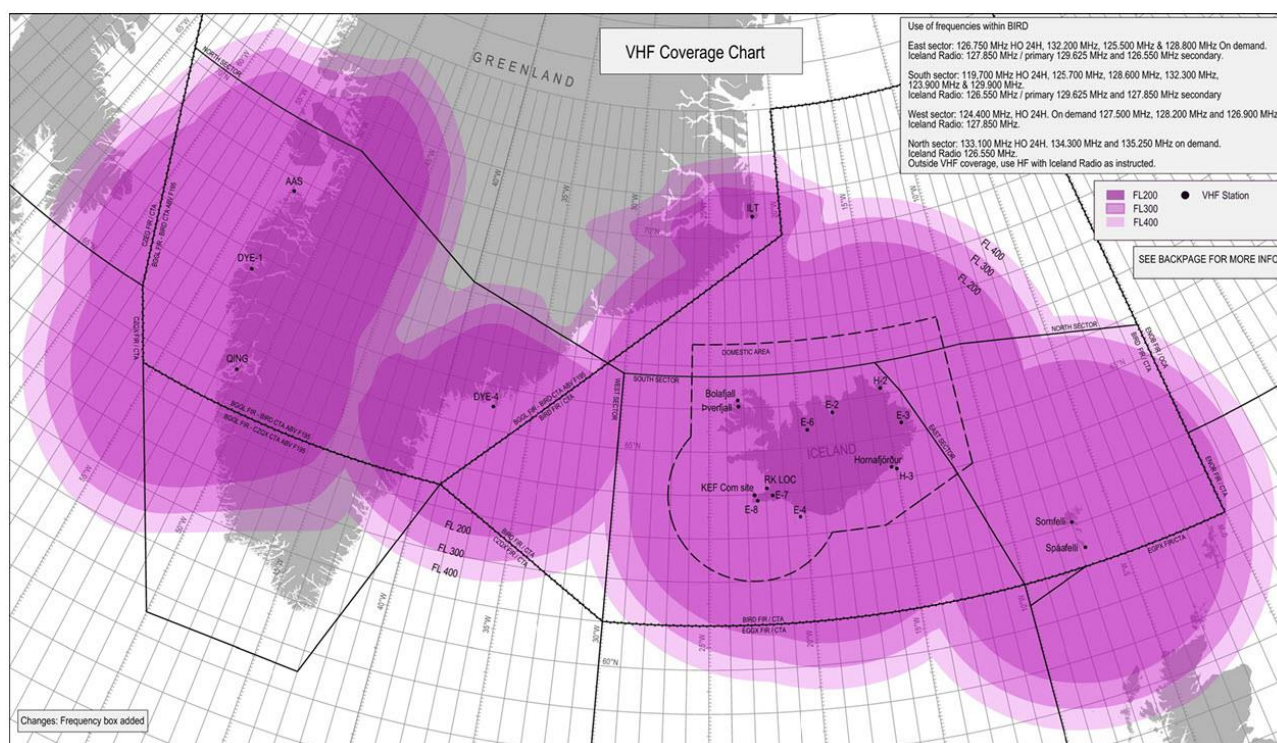
Figure 6-1 Reykjavik Control Direct Controller Pilot VHF Coverage
