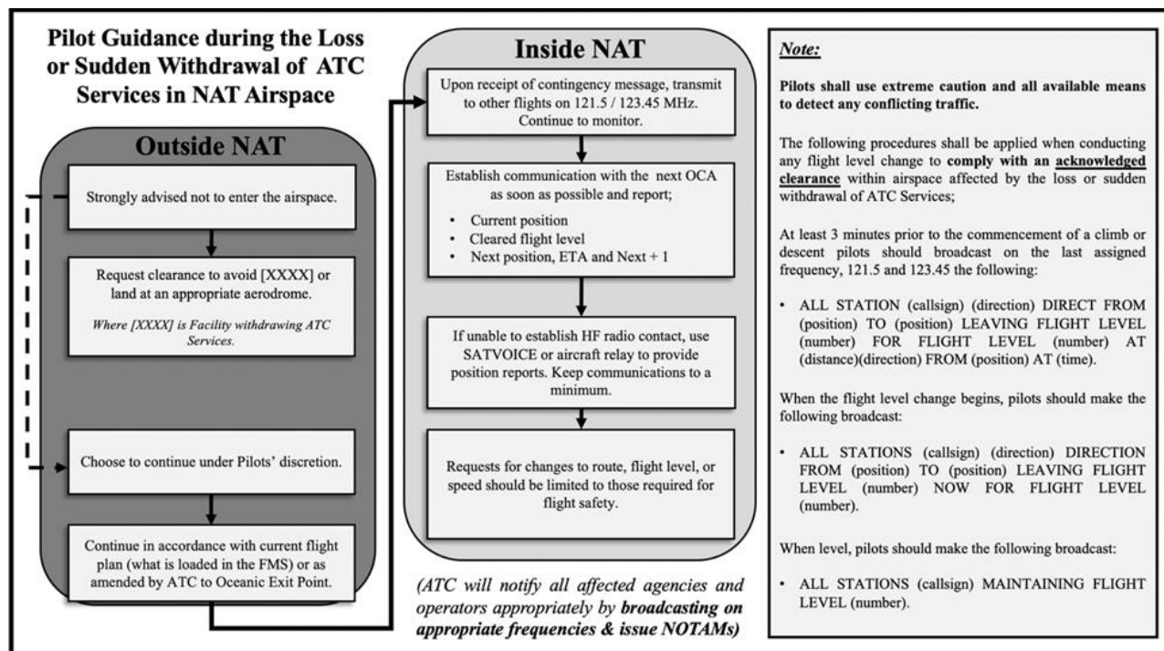
Figure 13-3 — Visual aid for pilot guidance during loss or sudden withdrawal of ATC services in NAT airspace.
